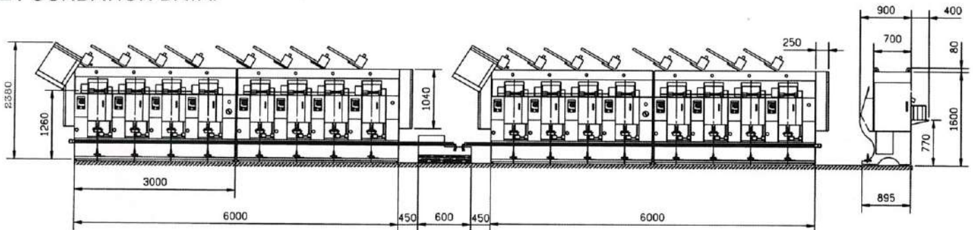
STANDARD TUBE TYPE BOBBIN MAGAZINE
